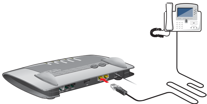
Connecting an IP telephone to the FRITZ!Box
